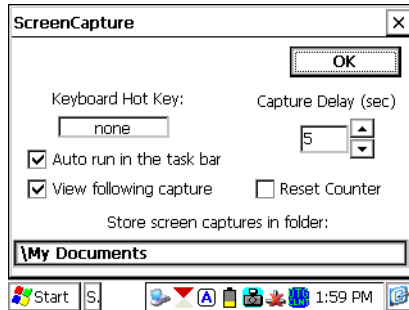
Figure 2-6. ScreenCapture Window
