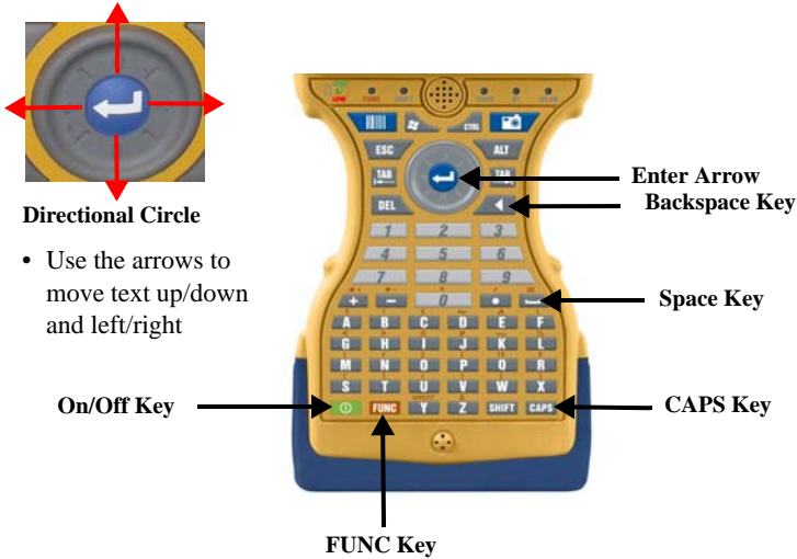
Figure 2-4. FC-2600 55-Key Keypad
